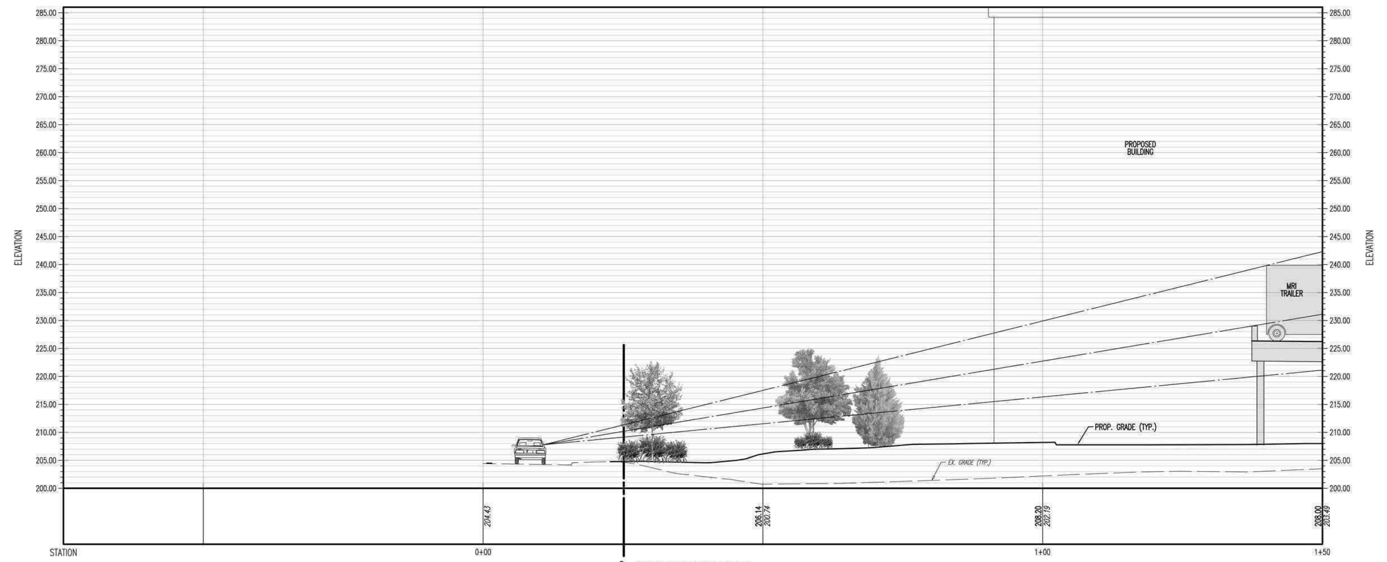
PROFILE VIEW OF SIGHT LINE 3 HORIZONTAL SCALE: 1"=10' VERTICAL SCALE: 1"=10'
